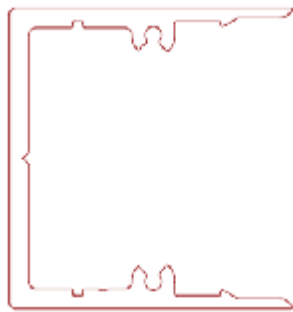
Click profile SQ 45 Mounting
